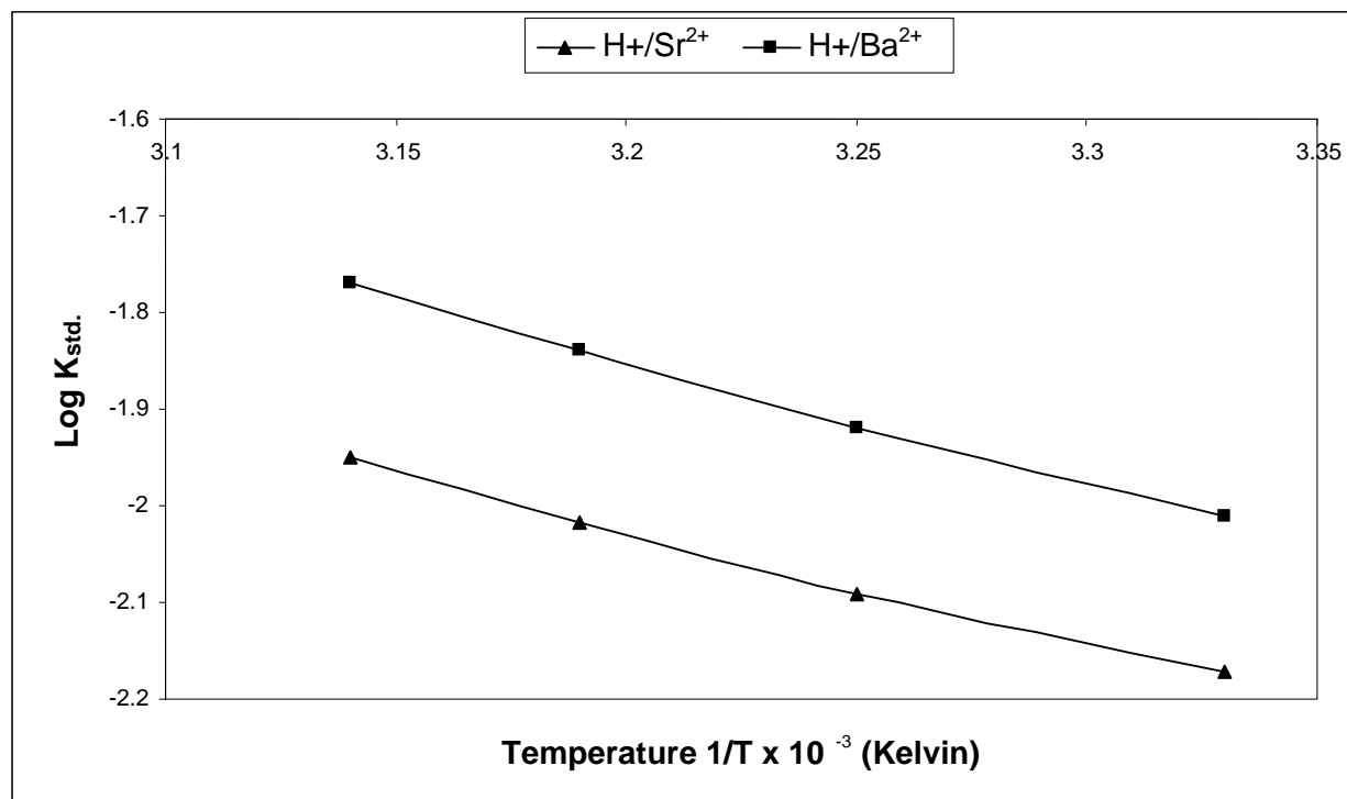
Fig.-1: Variation of Equilibrium Constant with Temperature for Uni-bivalent ion Exchange Reaction 1 and 2 Amount of ion exchange resin in H + form = 0.500g, Volume of exchangeable ion solution = 100.0 mL
