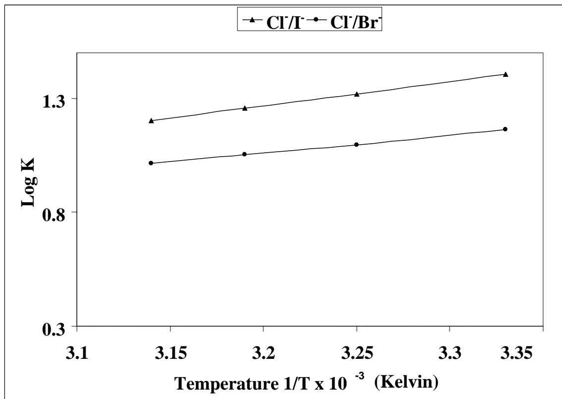
Fig.-1: Variation of Equilibrium Constant with Temperature for Uni-Univalent Ion Exchange Reactions using ion exchange resin Duolite 101-D
